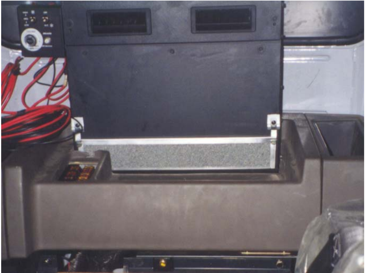
Evaporator in place on back wall of cab. Note that it extends above the lower window line.
